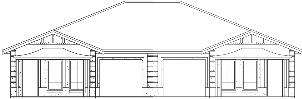
FRONT ELEVATION STYLE: VE1
